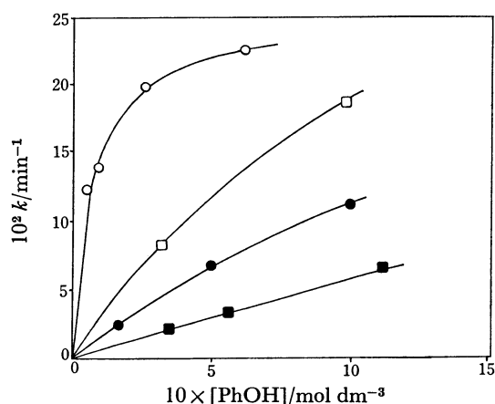
Fig. 1. Effect of [PhOH] on the first order rate constant k in various bpy concentrations for the reaction of 1 with phenol in THF at 23.2 °C. [bpy]=0 mol/dm 3 , ○; 0.90 × 10 -3 mol/dm 3 , □; 2.71 × 10 -3 mol/dm 3 , ●; 9.02 × 10 -3 mol/dm 3 , ■.
